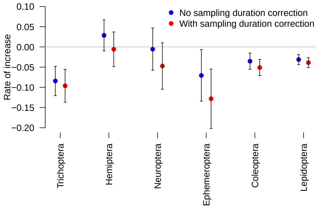
Supplementary Figure 2: Mean annual intrinsic rate of increase for each insect order based on data from De Kaaistoep, with and without correction for sampling time effort. Estimates are based on subset data for which information on sampling was available
