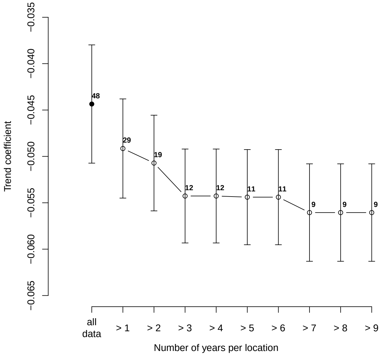
Supplementary Figure 3: Annual trend coefficient ( \pm 1\text{se} ) for subsets of the Wijster data. Each point depicts the trend as calculated for all locations that were sampled in more than x years. Numbers are the number of locations included in the data.
